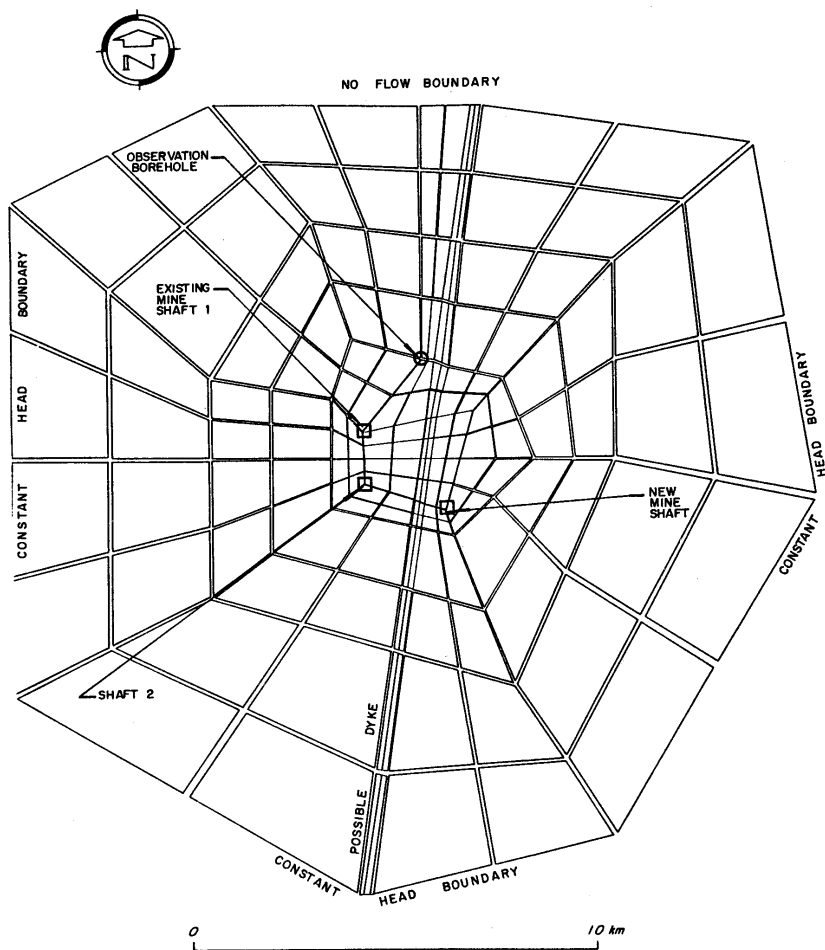
FIG 6 FINITE ELEMENT GROUND WATER MODELLING
