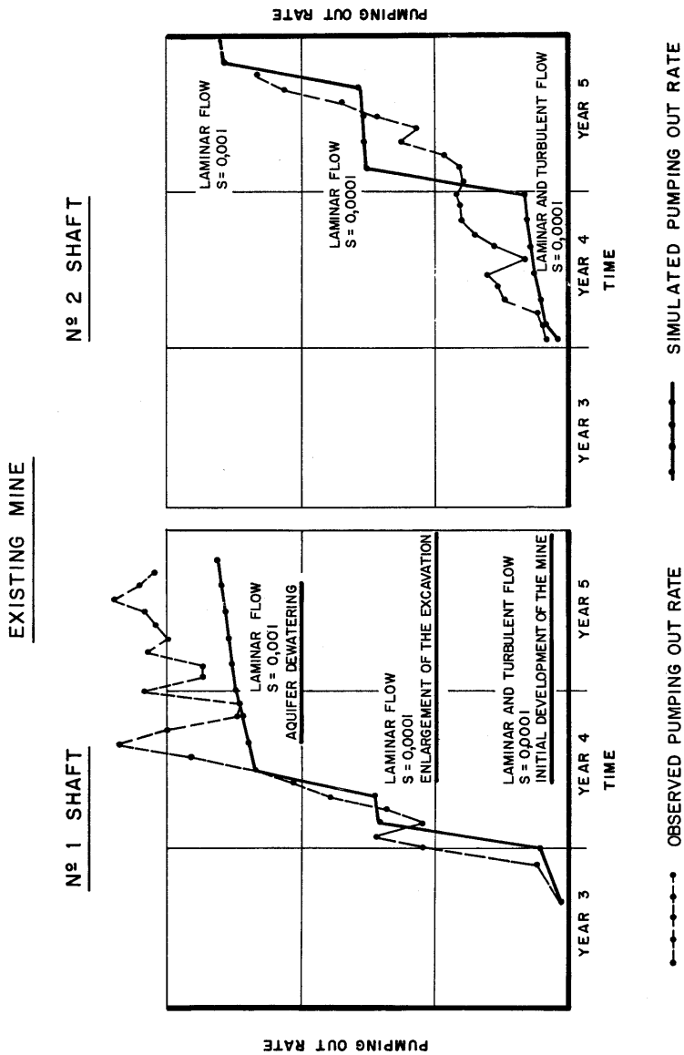
FIG 9 CALIBRATION OF INFLOW MODEL
